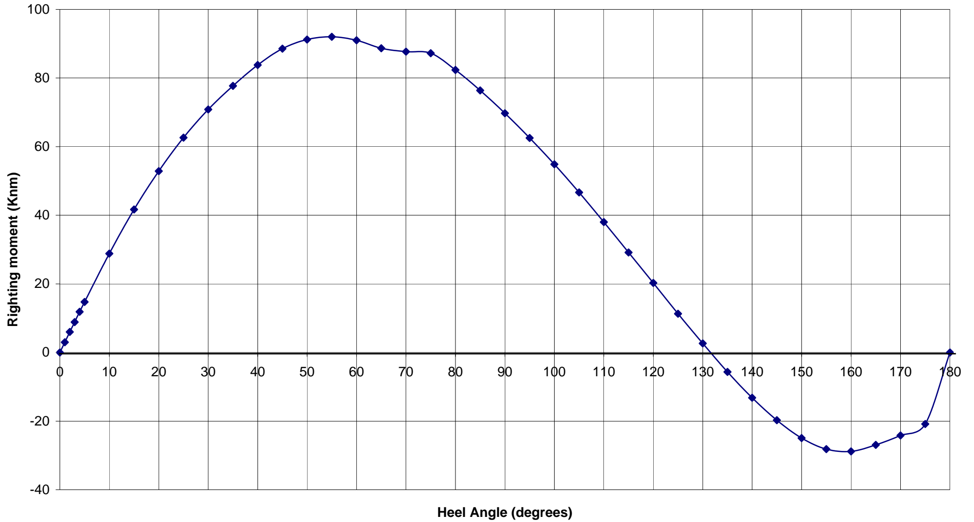
HYD155 Elan 450 Preliminary Rigthing moment data 140407 issue 1
